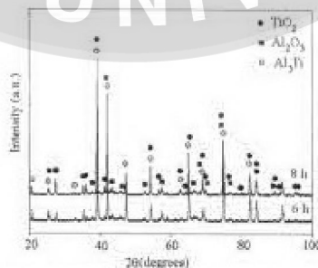
Figure 2 XRD patterns of Al-doped \text{TiO}_2 film for 6 h and 8 h
